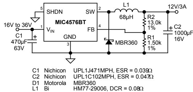
Figure 5. 16V–36V to 12V/3A Buck Converter Through Hole
