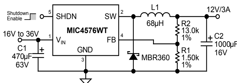
Adjustable Regulator
