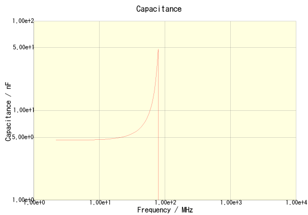
C2012C0G2A472J125AA
