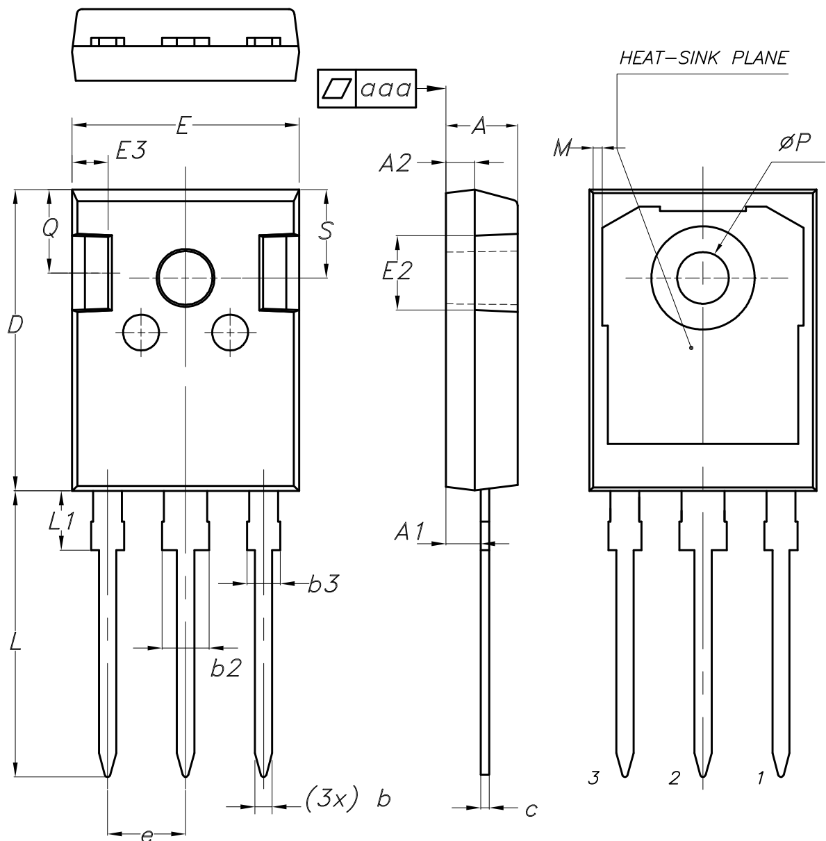
Figure 22. HiP247 long leads package outline
