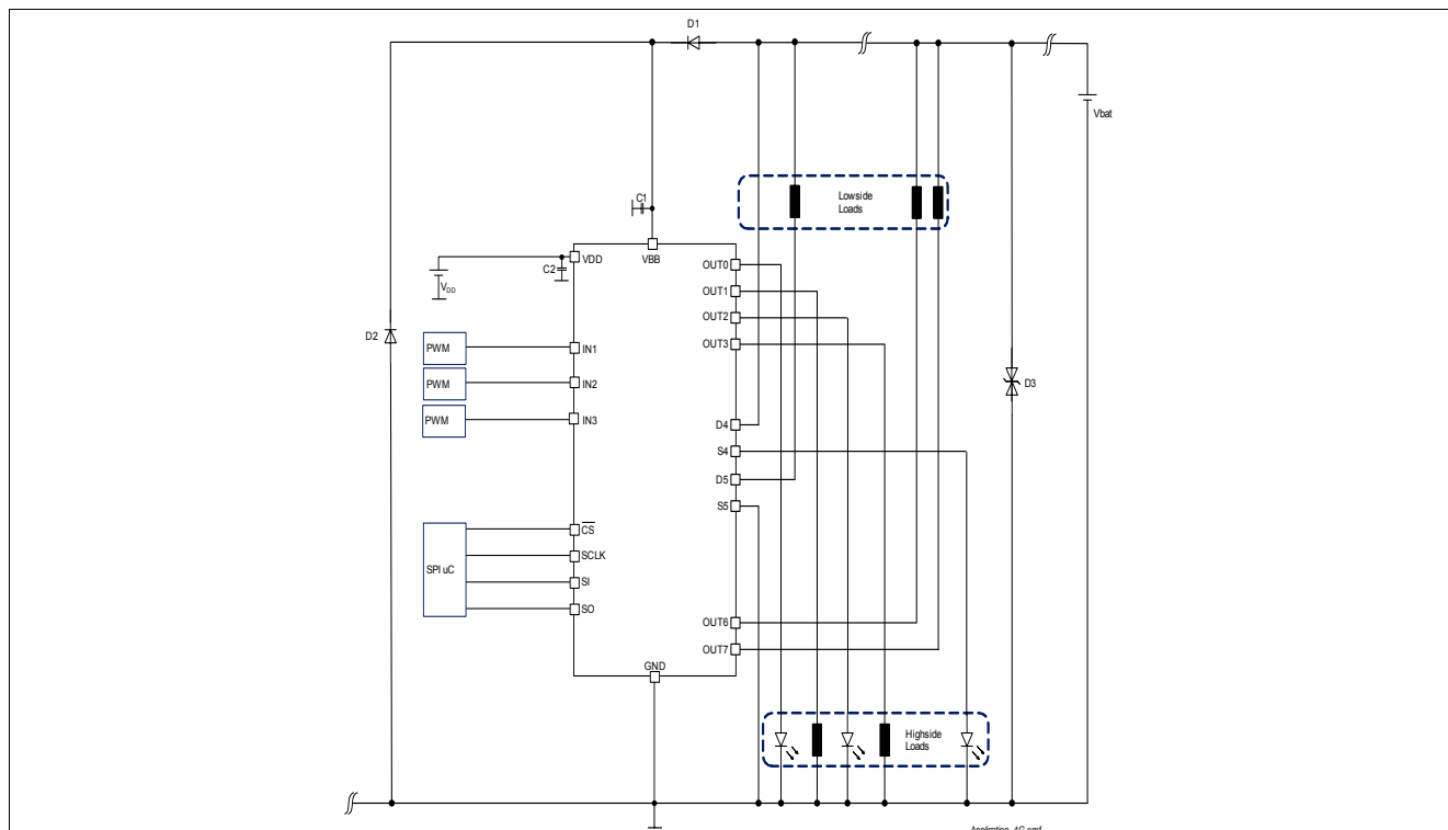
Figure 14 Application Diagram
