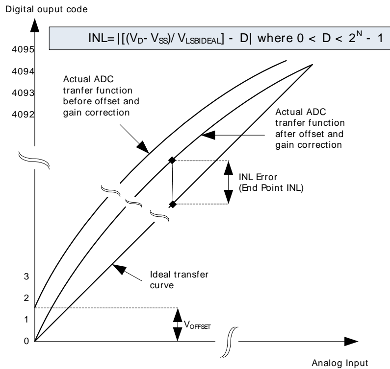
Figure 3.17. Integral Non-Linearity (INL)
