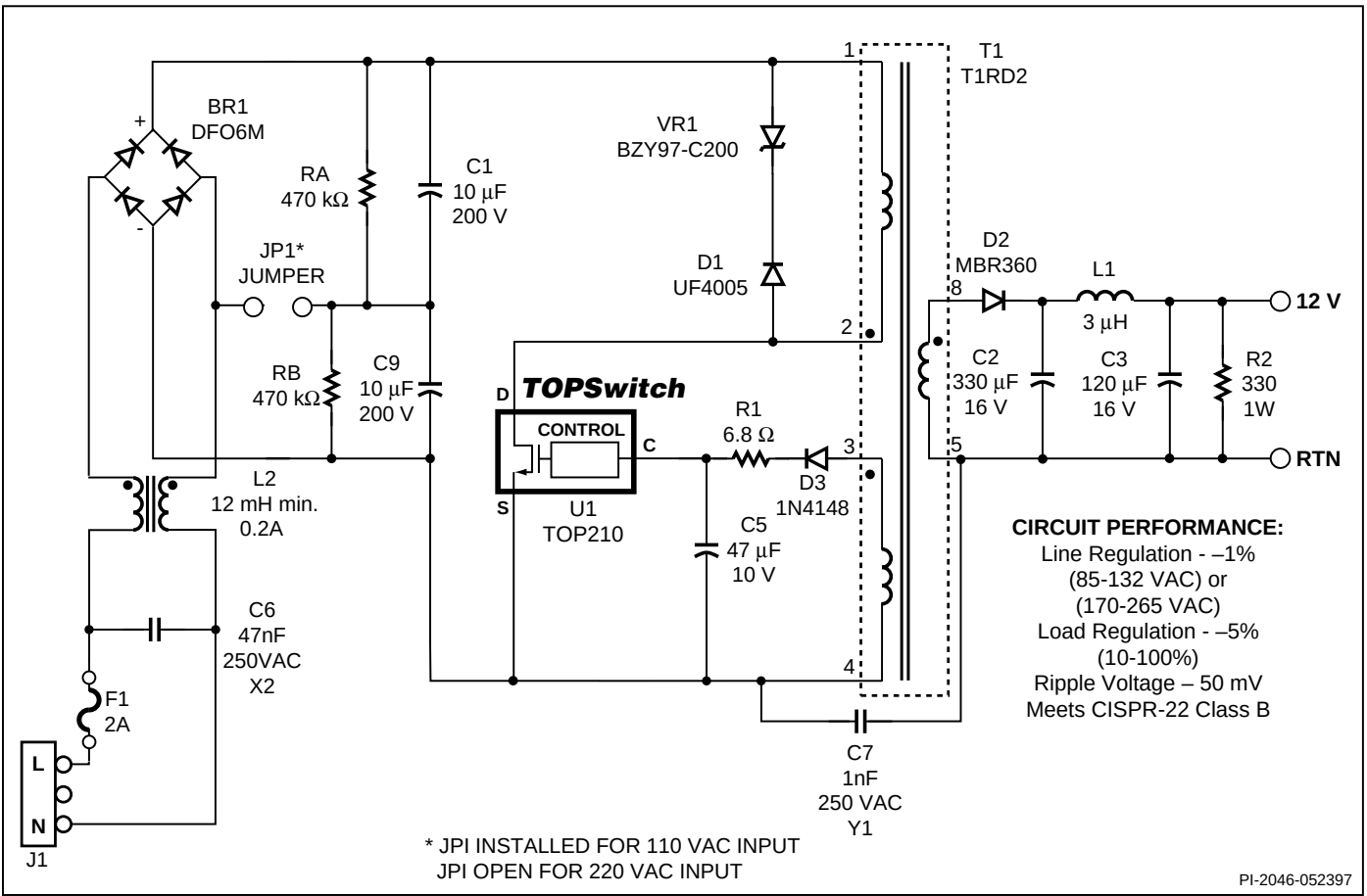
Figure 8. Schematic Diagram of a 12 V, 8 W 110/220 VAC Input Power Supply Using the TOP210.
