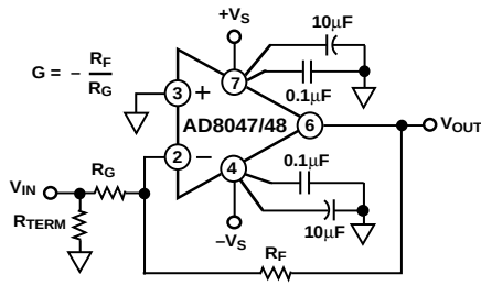
Figure 52. Inverting Operation
