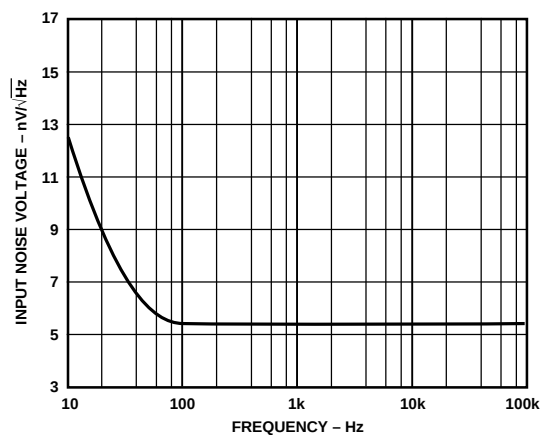
Figure 26. AD8047 Noise vs. Frequency
