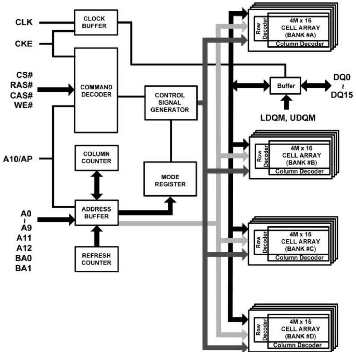
Figure 2. Block Diagram
