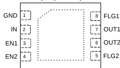
U-DFN3030-8
