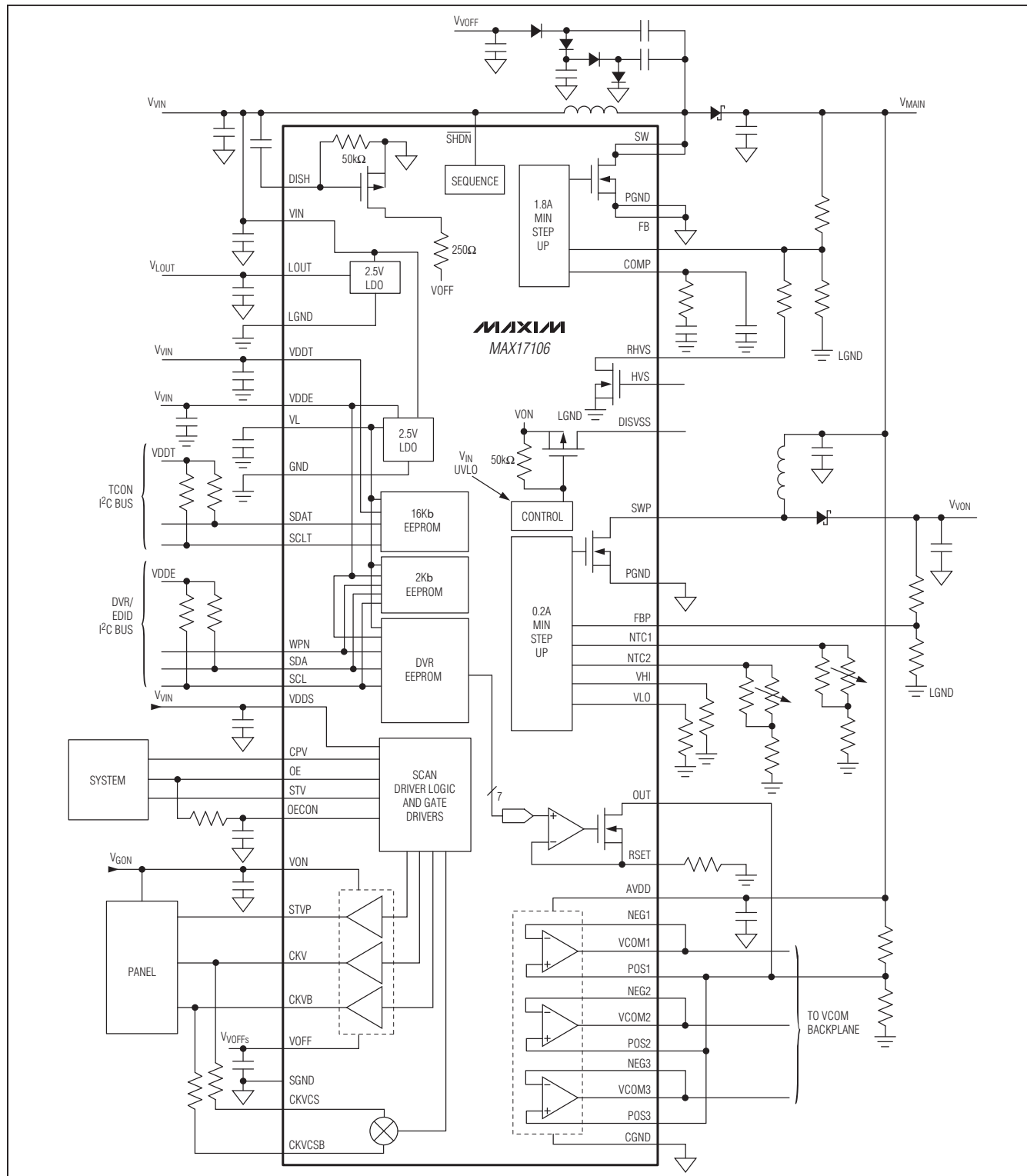
Figure 3. Functional Diagram
