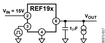
Figure 17. \overline{SLEEP} Response Time Measurement Circuit
