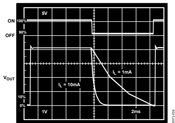
Figure 16. \overline{SLEEP} Response Time
