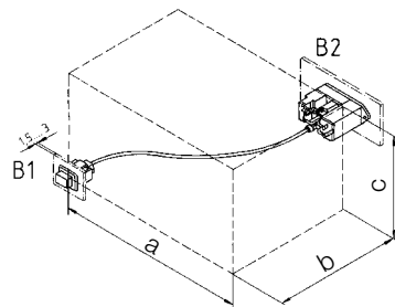
Slide clamp around cable Type R
