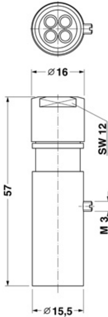
Dimensioned drawing
