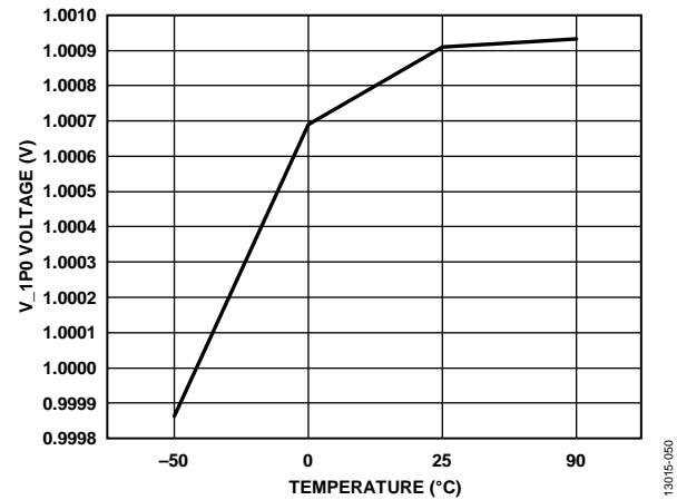
Figure 47. Typical V_1P0 Drift
