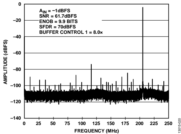
Figure 18. Single Tone FFT with f_{IN} = 1205.3 MHz
