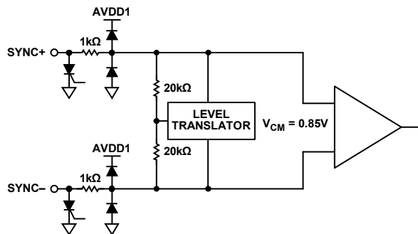
Figure 31. SYNC± Inputs
