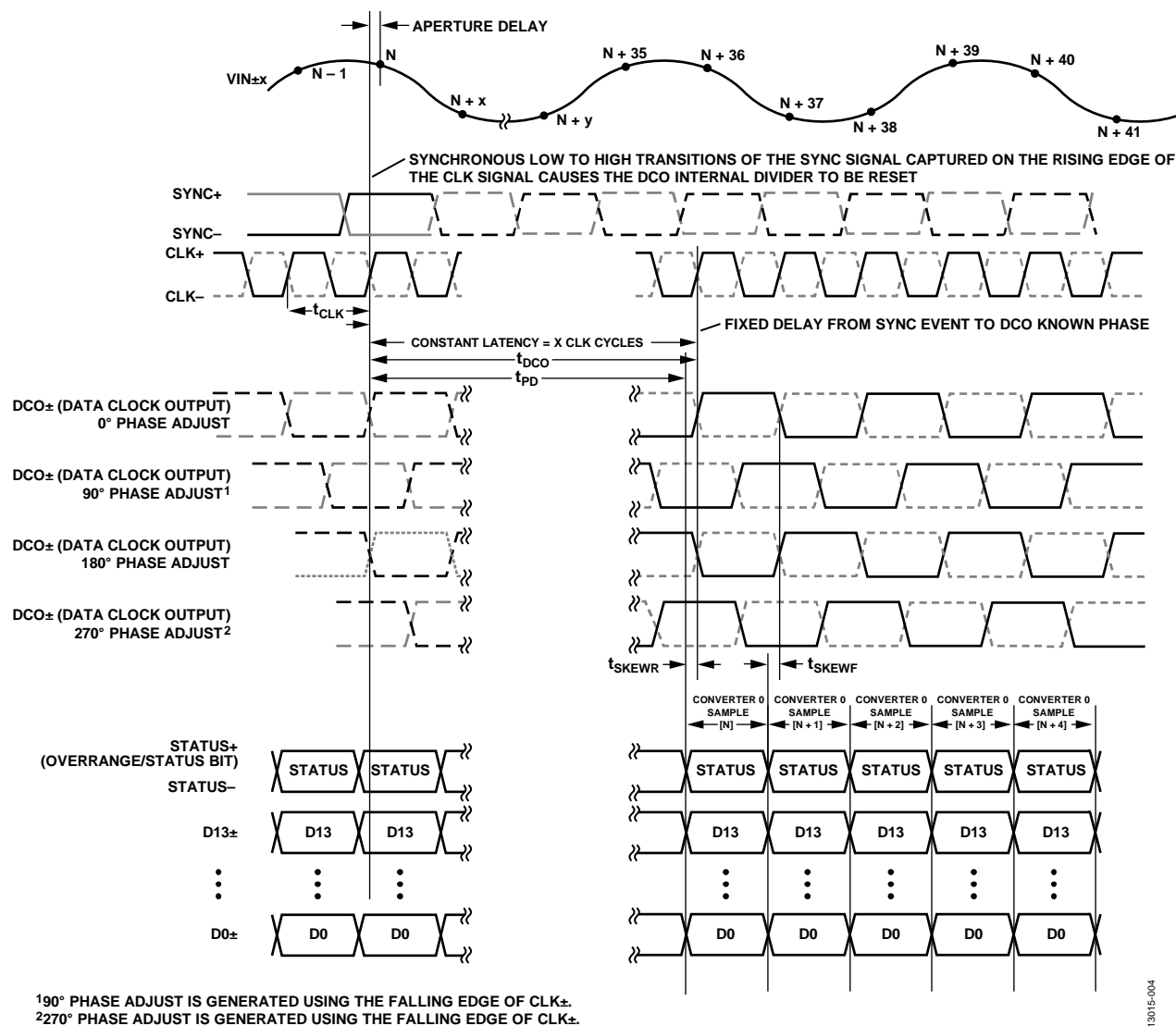
Figure 4. Parallel Interleaved Mode—One Converter, ≤14-Bit Data
