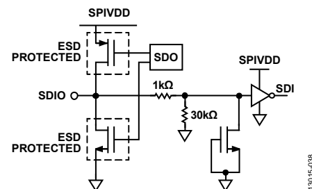
Figure 34. CSB Input
