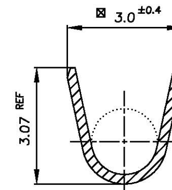
SECTION "C-C" Scale 10/1
