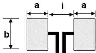
Recommended Pad Layout
