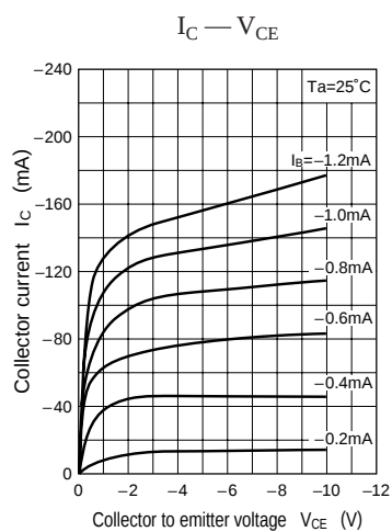
Characteristics charts of UN412Y
