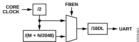
Figure 27. Fractional Divider Baud Rate Generation
