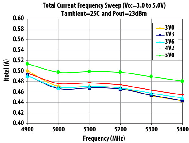
Figure 28. Total Current Frequency Sweep at 25C and Pout=23dBm over Vcc
