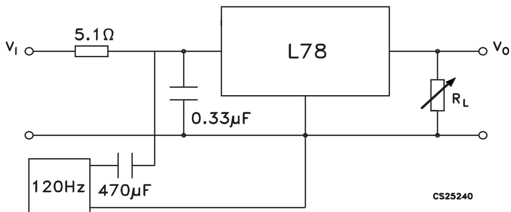
Figure 7. Ripple rejection
