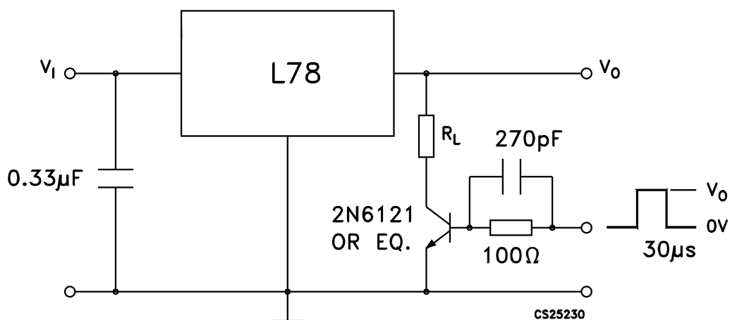
Figure 6. Load regulation
