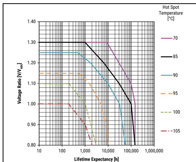
Lifetime Curve V_{NDC} = 600 V- and V_{NDC} = 700 V-
