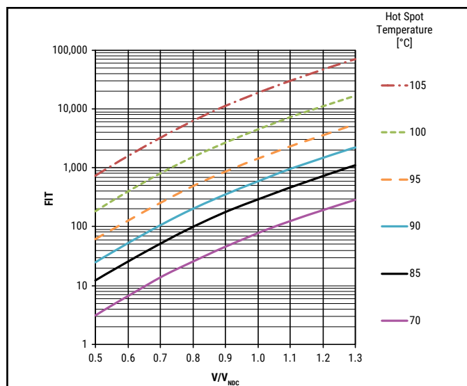
FIT at Hot Spot Temperatures
