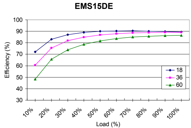
Figure 3. Efficiency, \eta (Line & load)
