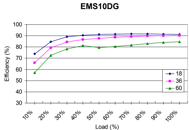
Figure 4. Efficiency, \eta (Line & load)
