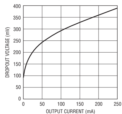
Dropout Voltage
