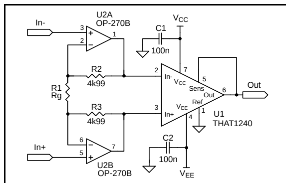
Figure 11. Instrumentation amplifier
