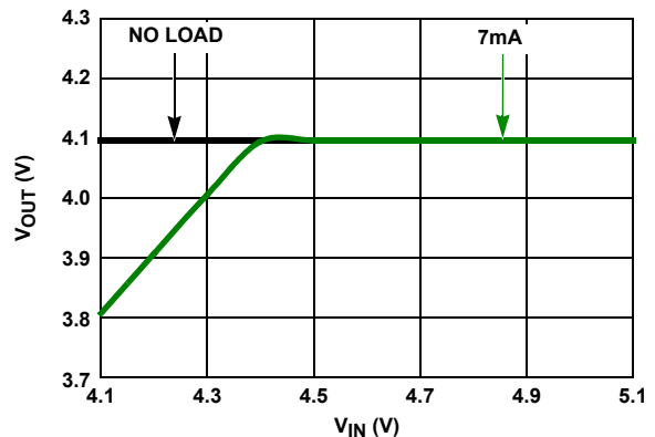
FIGURE 33. DROPOUT, ISL21080-41
