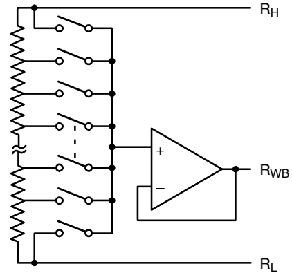
Figure 2. Electronic Potentiometer Implementation
