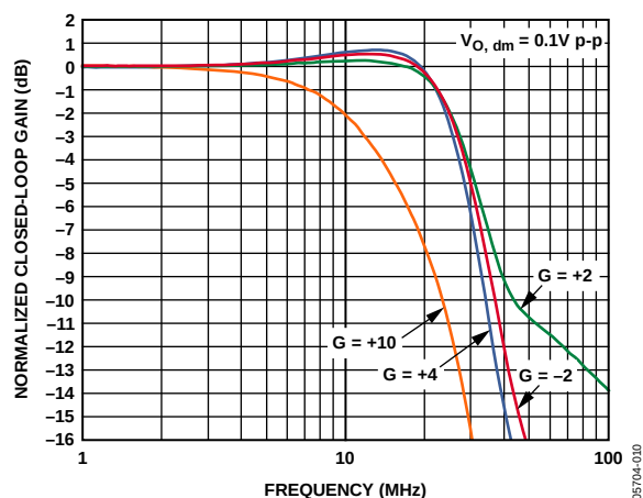
Figure 11. Small Signal Frequency Response for Various Gains
