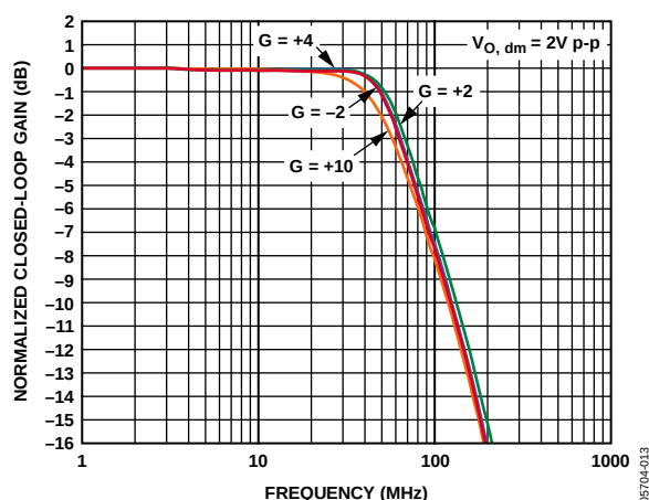
Figure 14. Large Signal Frequency Response for Various Gains
