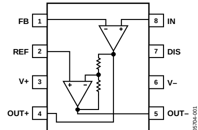
Figure 1. SOIC/LSCSP Pinout
