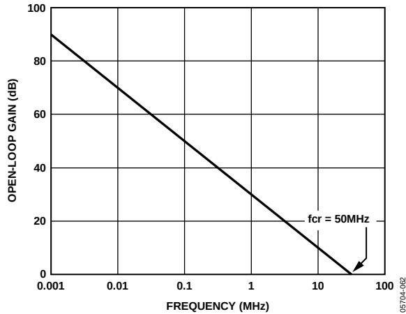
Figure 53. ADA4941-1 Op Amp Open-Loop Gain vs. Frequency
