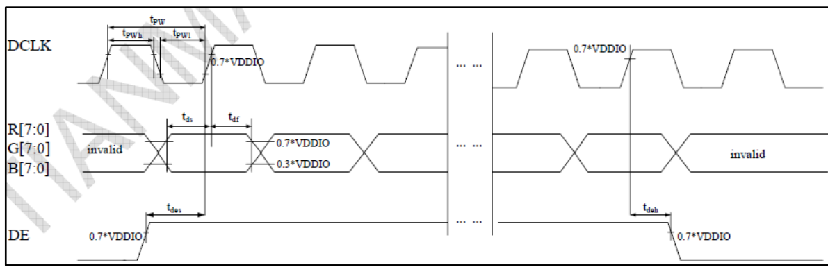
Figure 11 - Timing Diagram 2
