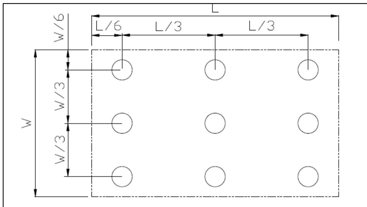
Figure 6 - Luminance measurement location
