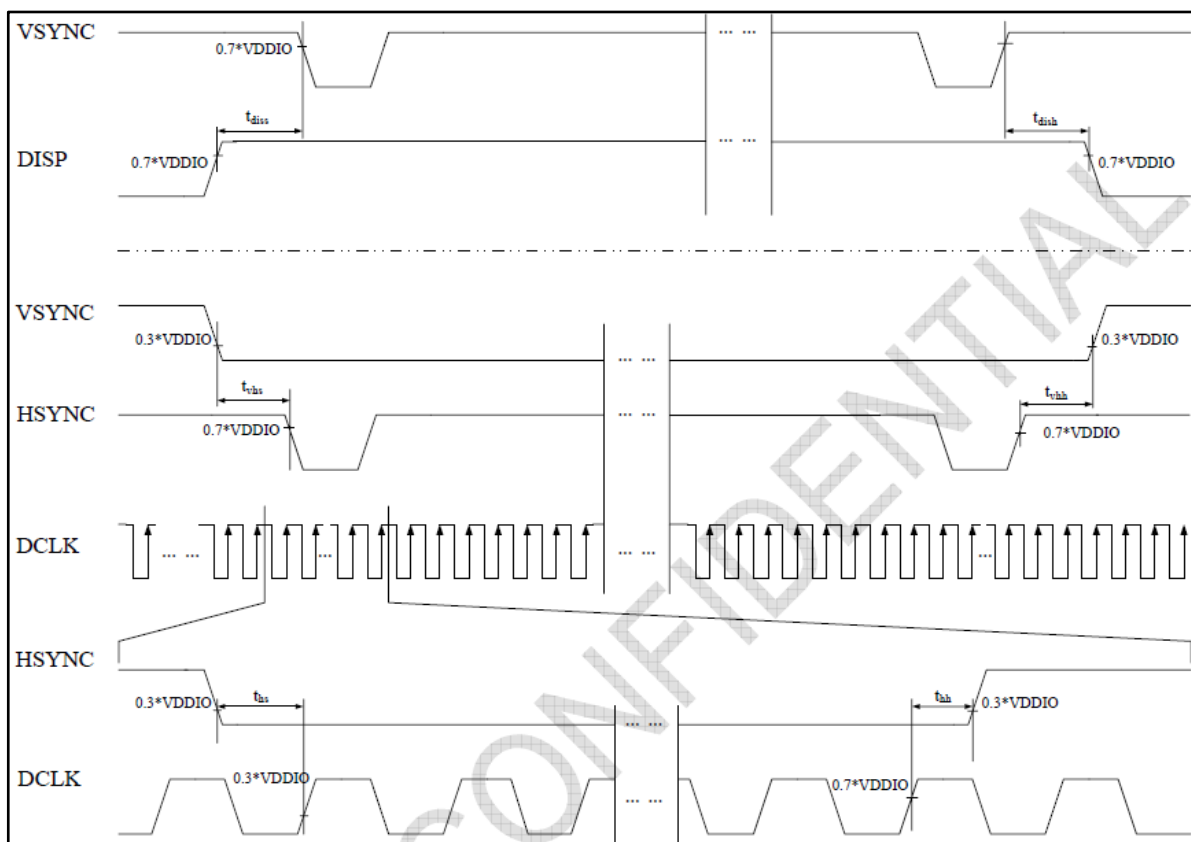
Figure 11 - Timing Diagram 2
