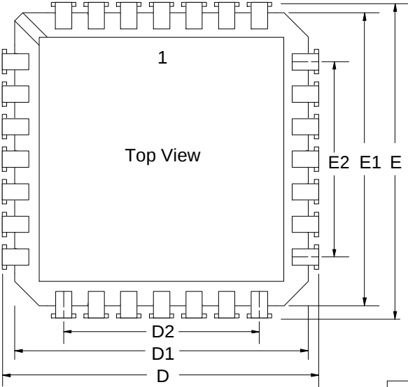
28/44 pin CLCC
