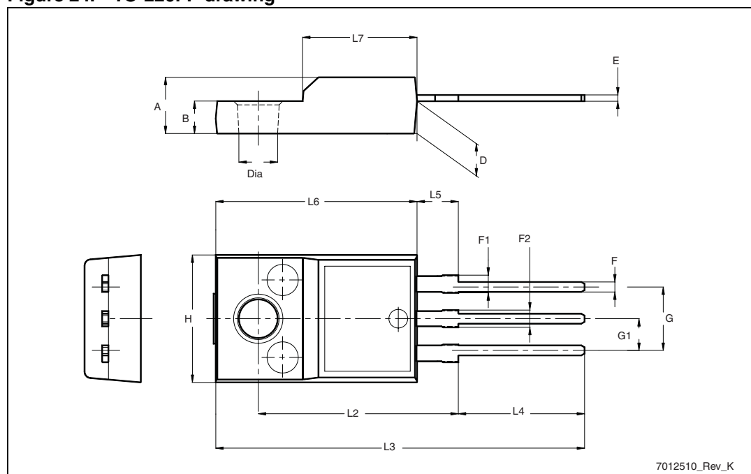
Figure 24. TO-220FP drawing
