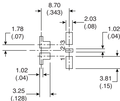
P.C. Mounting
