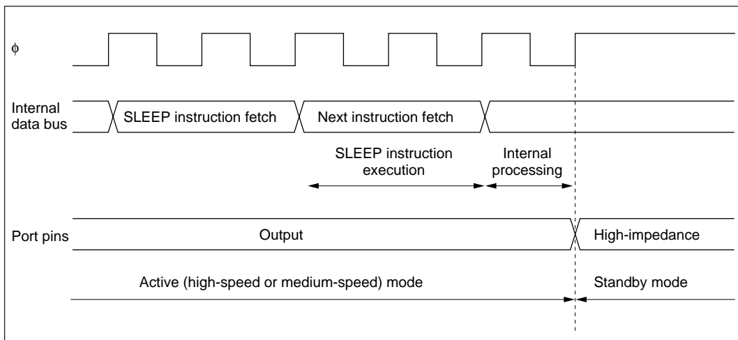
Figure 5-2 Transition to Standby Mode and Port Pin States
