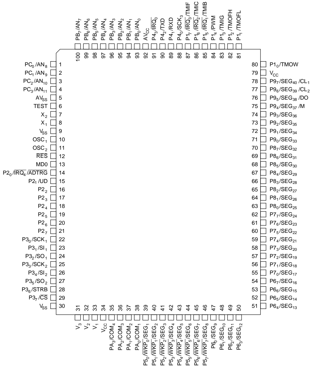
Figure 1-3 Pin Arrangement (FP-100A: Top View)
