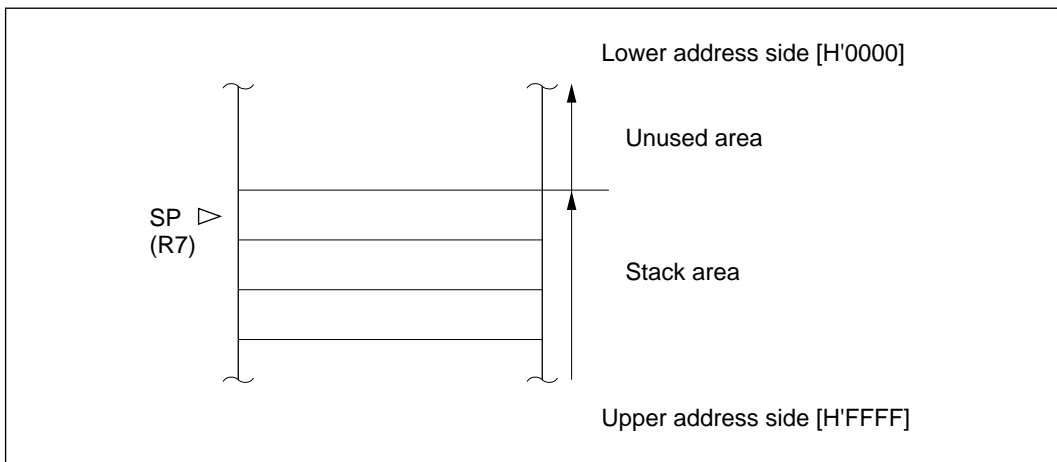
Figure 2-2 Stack Pointer
