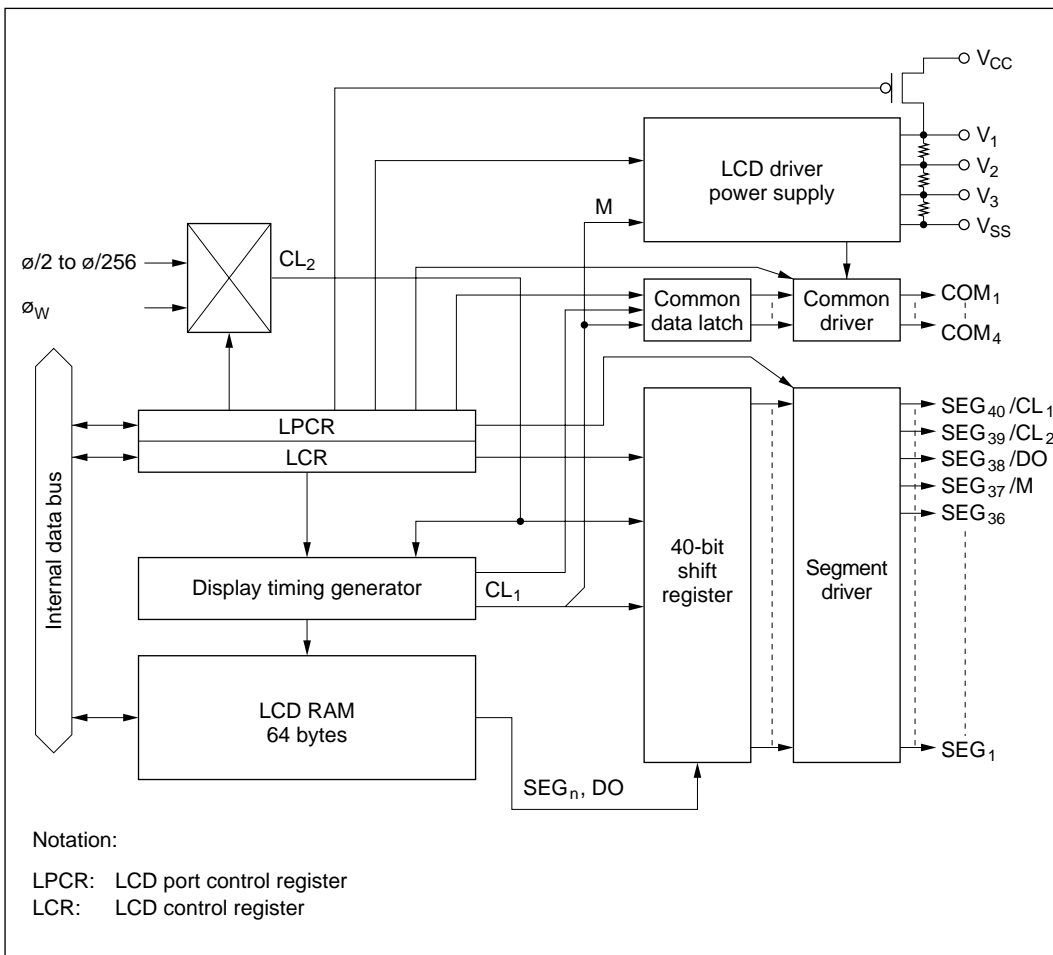
Figure 13-1 LCD Controller/Driver Block Diagram
