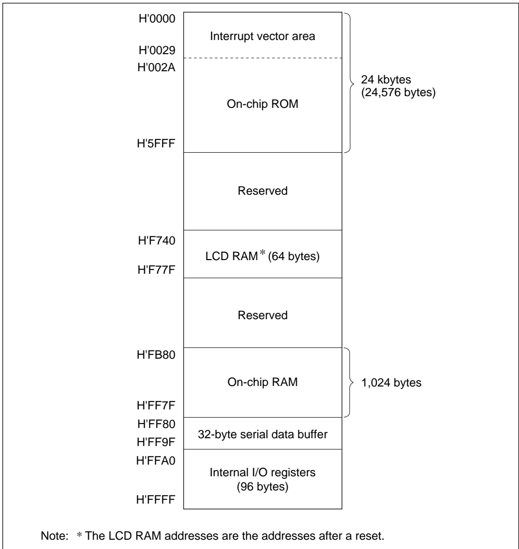
Figure 2-16 (a) H8/3833 Memory Map
