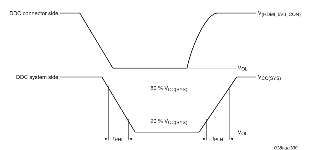
Fig 14. Transition time DDC system side
