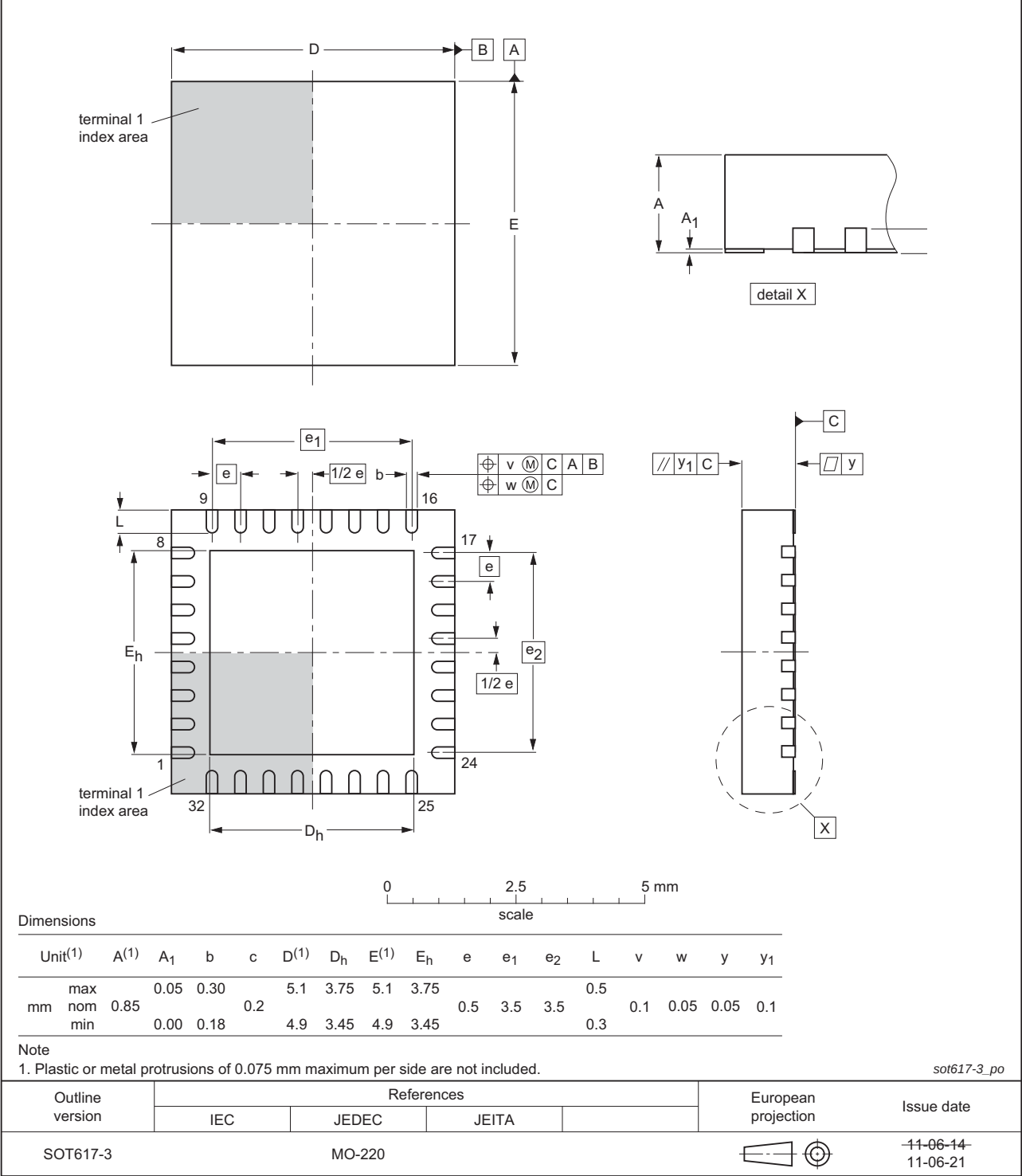
Fig 25. Package outline DFN5050-32 (SOT617-3/HVQFN32)
