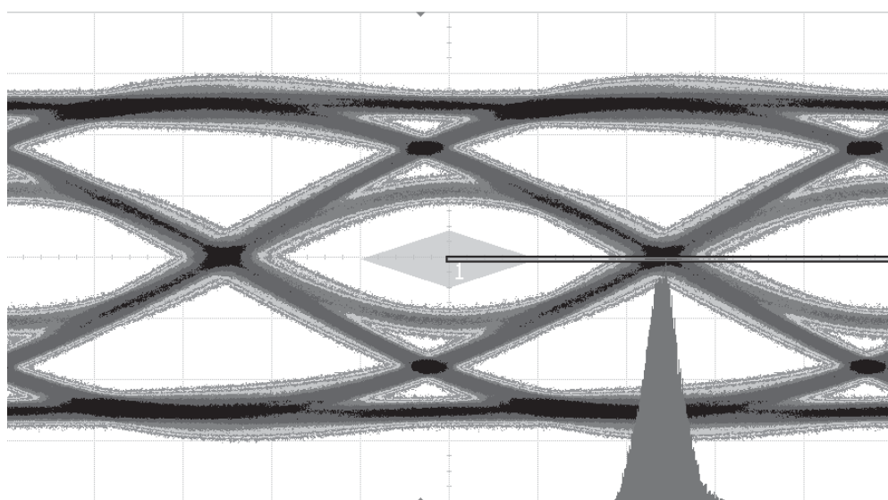
Fig 5. Eye diagram using IP4788CZ32 (1080p, 16 bit)
