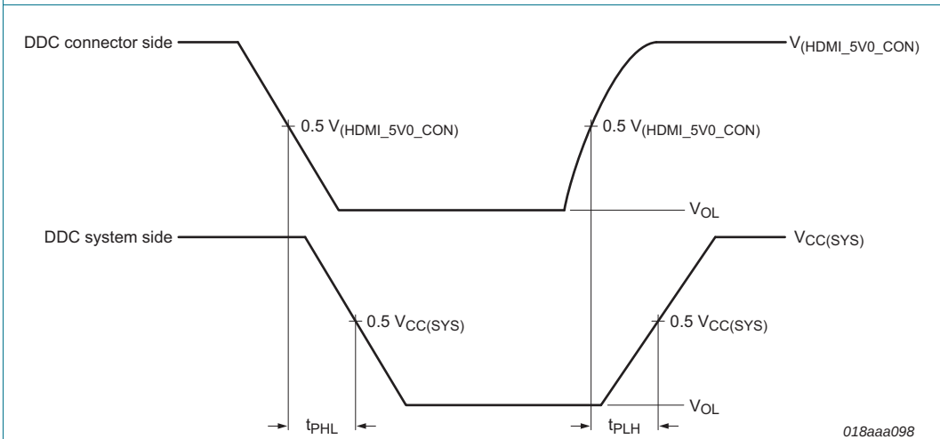
Fig 12. Propagation delay DDC, DDC connector side to DDC system side
