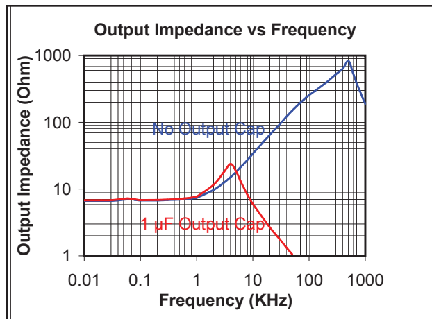
Output Impedance
