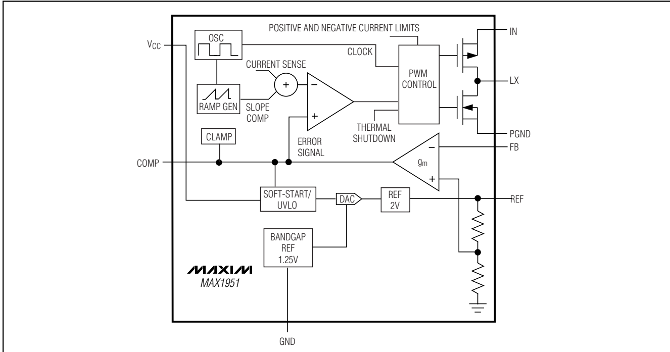
Figure 1. Functional Diagram
