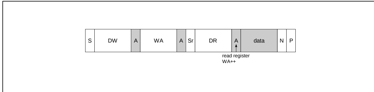
Figure 23. Random Read
