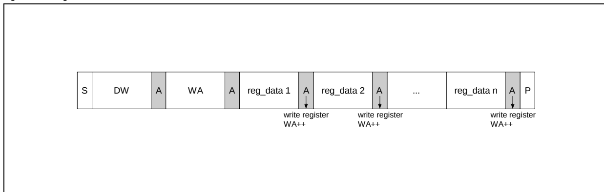
Figure 22. Page Write
