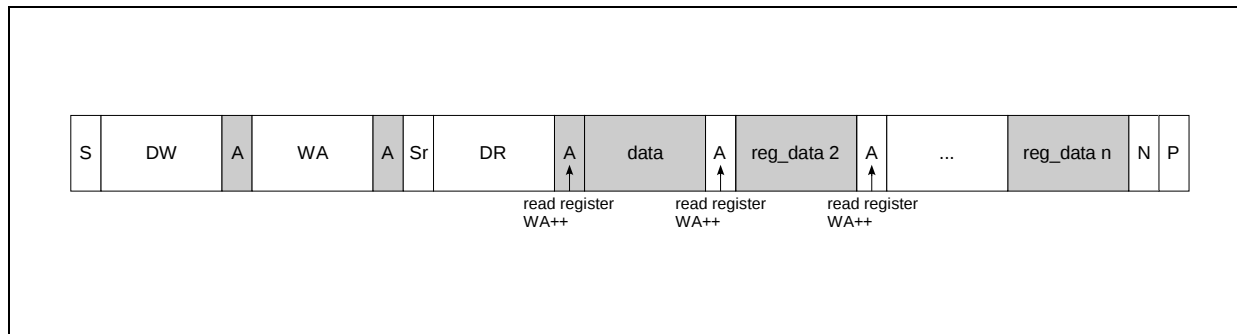
Figure 24. Sequential Read
