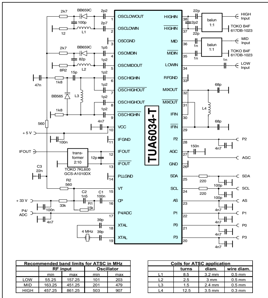
Figure 7 Application Circuit TUA6034-T for ATSC
