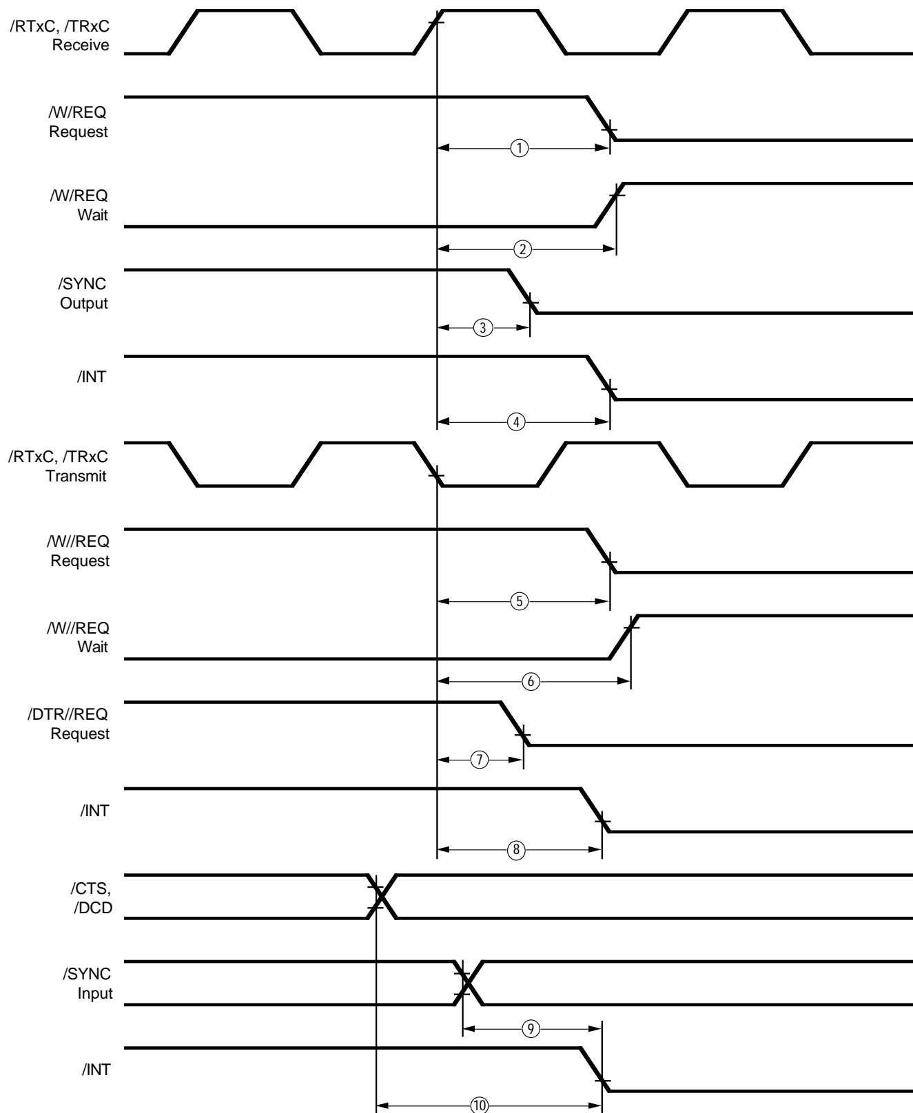
System Timing
