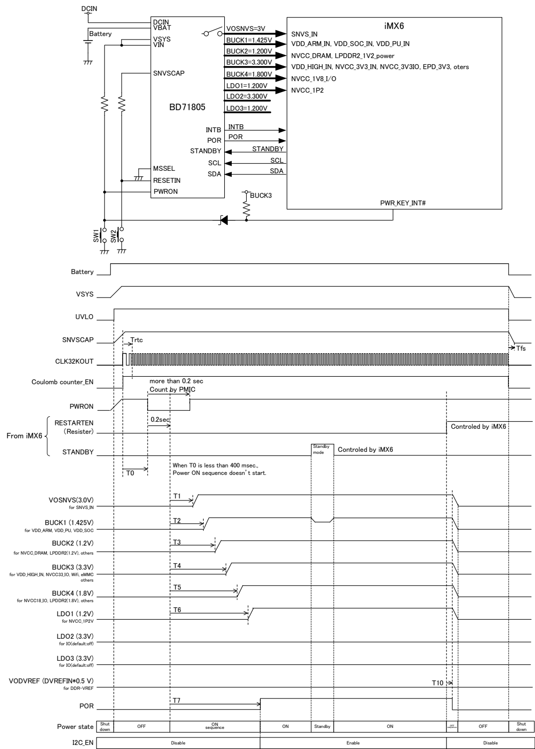
Figure 14. Power-ON/OFF Sequence (Master control mode)
