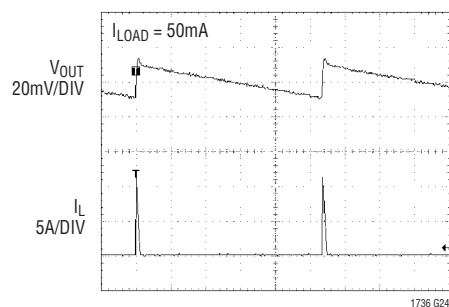
V_{OUT}(\text{RIPPLE}) (Burst Mode Operation)
