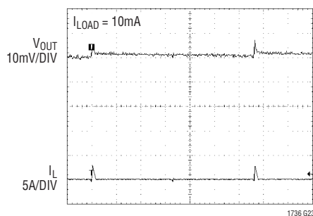
V_{OUT}(\text{RIPPLE}) (Synchronized)
