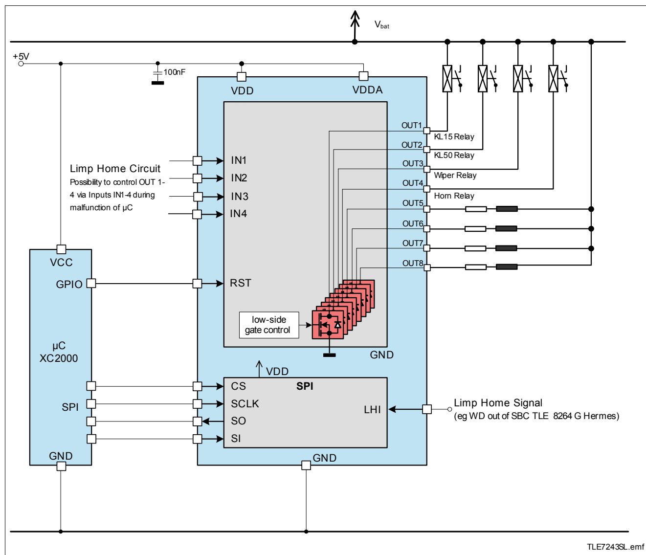
Figure 13 Application Diagram
