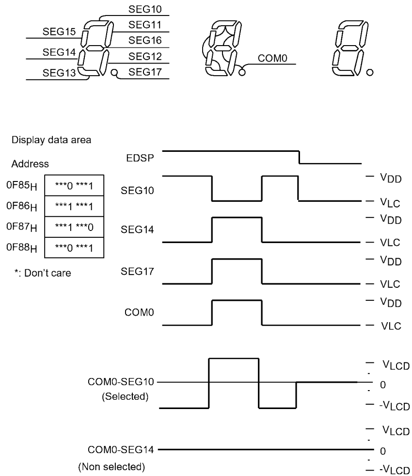
Figure 15-11 Static Drive
