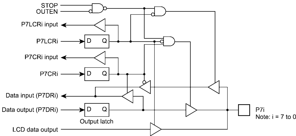
Figure 5-7 Port P7
