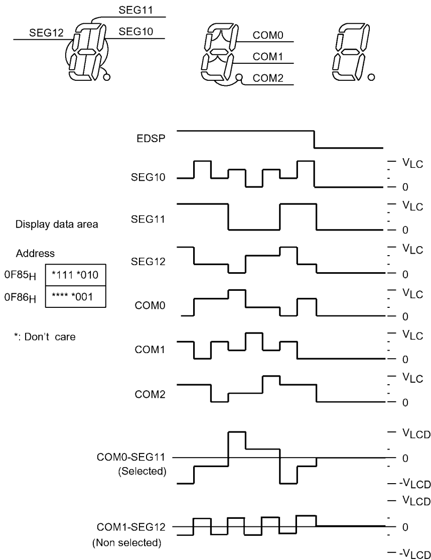
Figure 15-8 1/3 Duty (1/3 Bias) Drive
