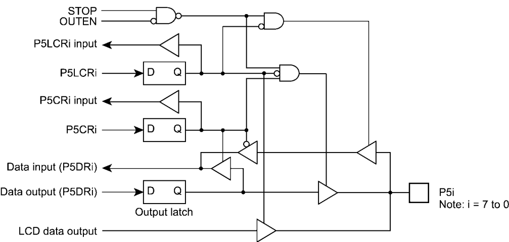
Figure 5-5 Port P5
