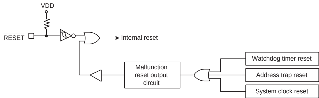
Figure 2-15 Reset Circuit
