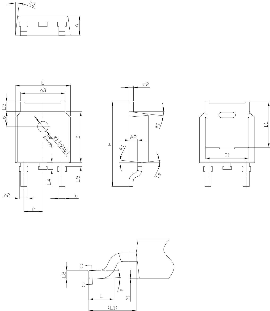
Figure 25. DPAK (TO-252) type C3 package outline
