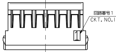
VIEW "H"
