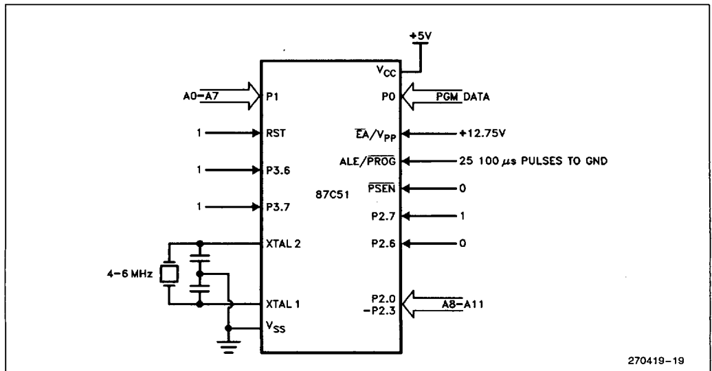
Figure 11. Programming Configuration
