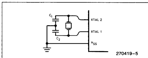
Figure 4. Using the On-Chip Oscillator
