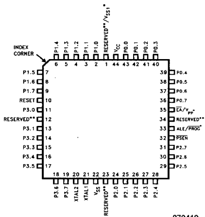
Pad (PLCC)
