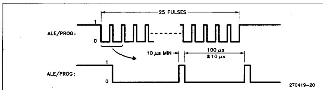
Figure 12. PROG Waveforms
