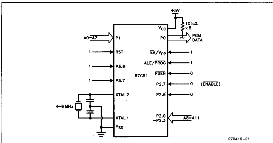
Figure 13. Program Verification
