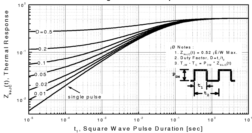
Fig 11. Thermal Response
