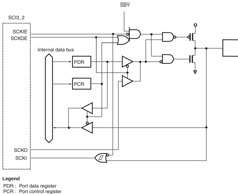
Figure B.21 Port 7 Block Diagram (P70)
