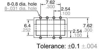
Recommended mounting pad (TOP VIEW)
