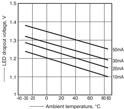
4. LED dropout voltage vs. Ambient temperature characteristics LED current: 10 to 50 mA
