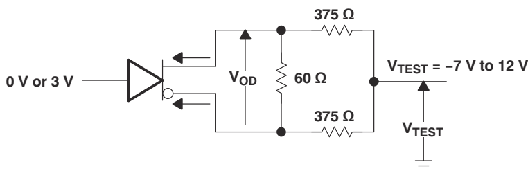
Figure 8-2. Driver Test Circuit, V_{OD} With Common-Mode Loading
