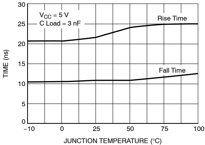
Figure 9. DRVH Rise and Fall Times vs. Temperature
